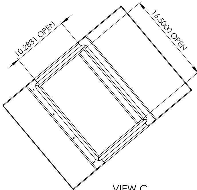
VIEW C SCALE 1 : 10
